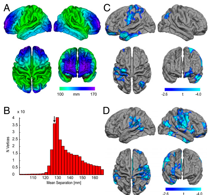
Fig. 2. (A) MSDs for points on the cortical surface, averaged across controls. (B) Distribution of MSDs across the cortical surface. The arrow indicates the average of the distribution (i.e., “mean geodesic”). (C) Random-field, theory-based, cluster-corrected ( P < 0.01 ) difference map showing significantly reduced MSDs in ASD relative to controls. (D) Clusters of significant negative correlations between MSDs and the repetitive domain of the ADI-R within the ASD group (RFT-based, cluster-corrected, P < 0.01 ). r_{\text{neg}} , negative correlation coefficient; t , statistical test parameter for correlation coefficient.
