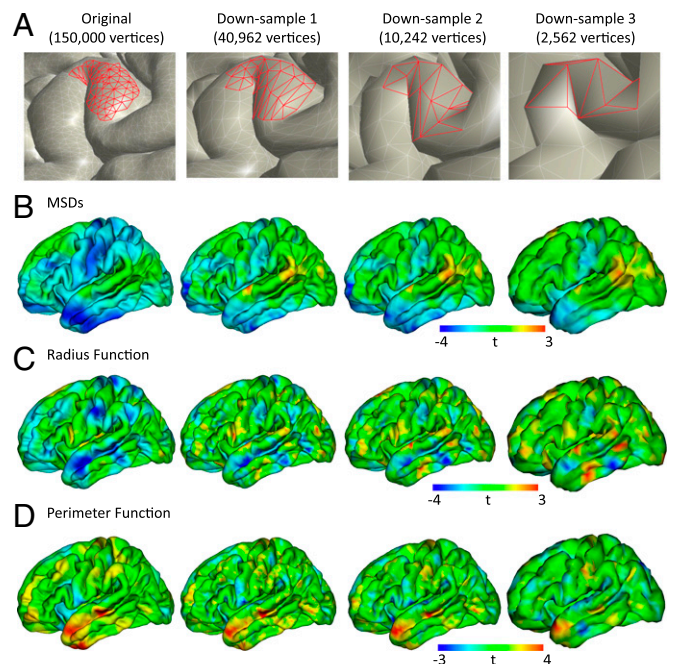
Fig. 4. (A) Cortical mesh patterning of the original high-resolution pial surface and of three standard templates with decreasing levels of resolution. The vertices delineated are roughly within the same location and illustrate the degree of detail lost at each successive iteration. (B–D) Difference maps (t statistic) between individuals with ASD and controls for mean separation distances (B), intraareal wiring costs (C), and interareal wiring costs (D). Negative t values (green to blue) indicate smaller parameter values in ASD relative to controls whereas positive t values (green to red) indicate larger parameter values in ASD.
