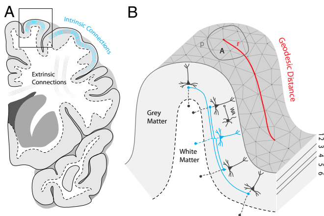
Fig. 1. (A) Schematic diagram illustrating the intrinsic horizontal connectivity of the cortex including long-range intrinsic axon collaterals of pyramidal neurons (cyan) and terminals of wide-arbor (WA) inhibitory basket cells. (B) Geodesic mesh consisting of points (i.e., vertices) characterizing the cortical surface. The geodesic distance (marked in red) is the shortest path along the surface that connects two surface points. Circle indicates geodesic circle of area A, radius r , and perimeter p .
