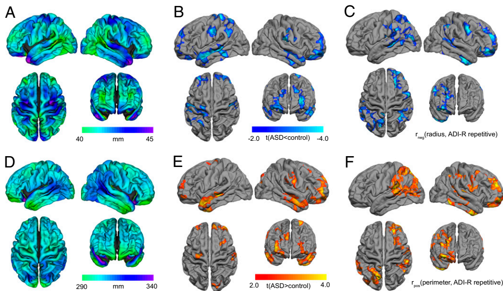
Fig. 3. (A) Intraareal wiring-cost function (referred to as the radius function) of the cortex at a scale of 5% averaged across controls. (B) Random-field, theory-based, cluster-corrected ( P < 0.05 ) difference map indicating regions with reduced radii in ASD relative to controls. (C) Clusters of significant negative correlations ( P < 0.05 ) between radius function and the severity of autistic symptoms in the repetitive domain. (D) Interareal wiring-cost function (referred to as the perimeter function) averaged across controls at a scale of 5%. (E) Clusters (RFT-based, cluster corrected, P < 0.05 ) with enhanced perimeters in ASD relative to controls. (F) Clusters (RFT-based, cluster-corrected, P < 0.05 ) of significant positive correlations between perimeter and the severity of autistic symptoms in the repetitive domain.
